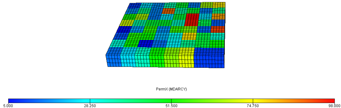
Figure 1 Permeability Map, Reservoir Dimension
